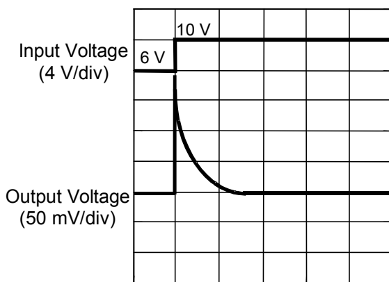
Figure 15 Ringing Waveform of Power Supply Variation (VOUT Pin)
