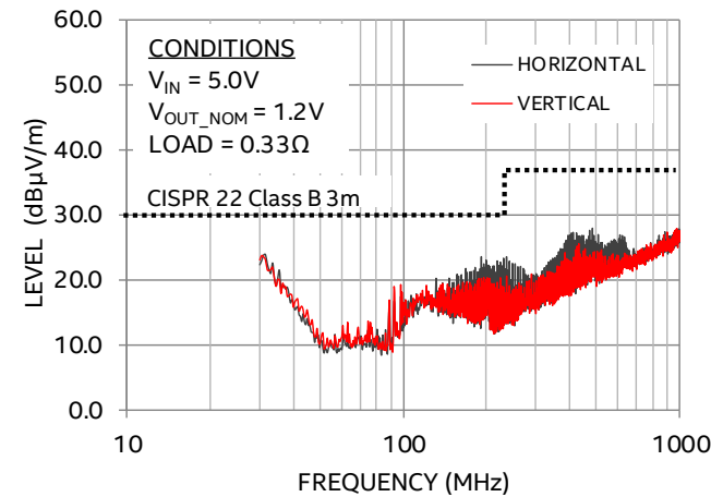
EMI Performance
