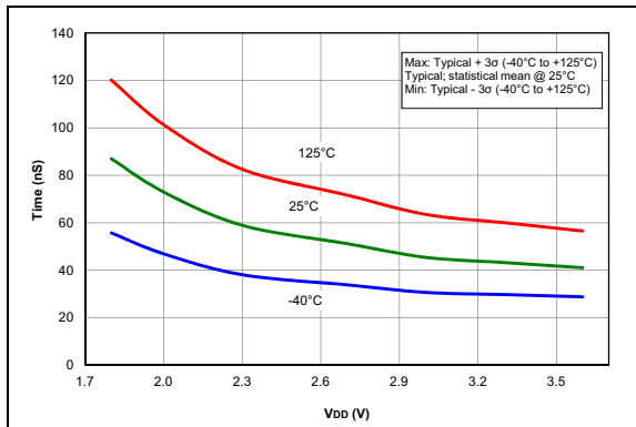
FIGURE 38-68: Comparator Response Time Over Voltage, NP Mode ( CxSP = 1 ), Typical Measured Values, PIC16F18855/75 Only.
