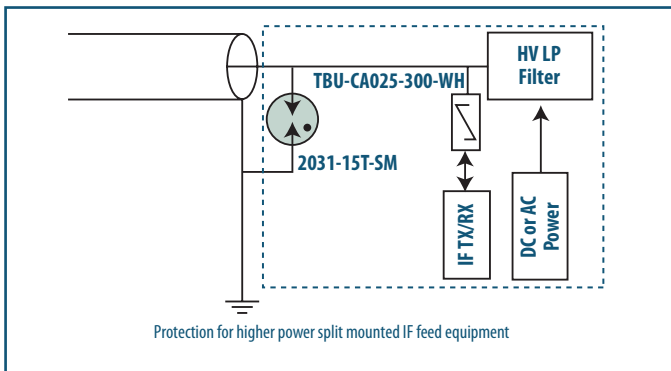
Microwave Link
