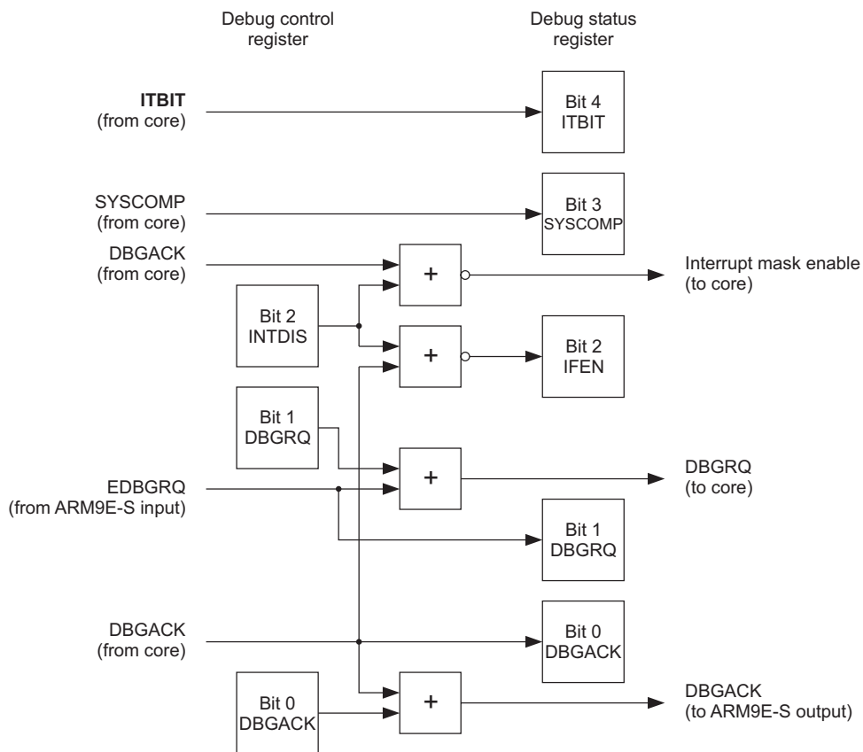
Figure C-12 Debug control and status register structure
