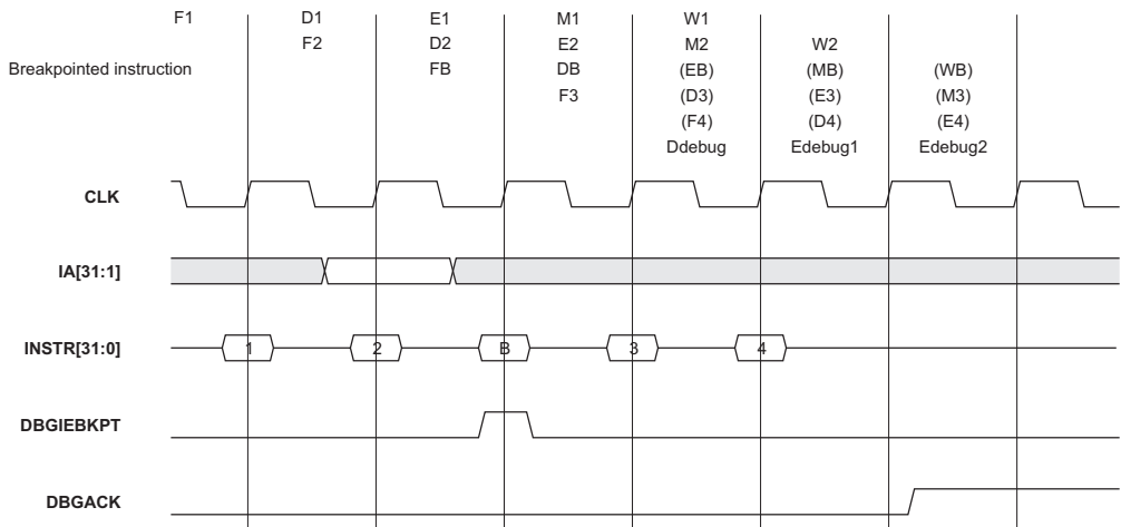
Figure 7-4 Breakpoint timing
