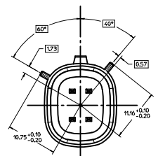
KEYING OPTION C SCALE 4:1
