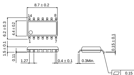
SOP14
