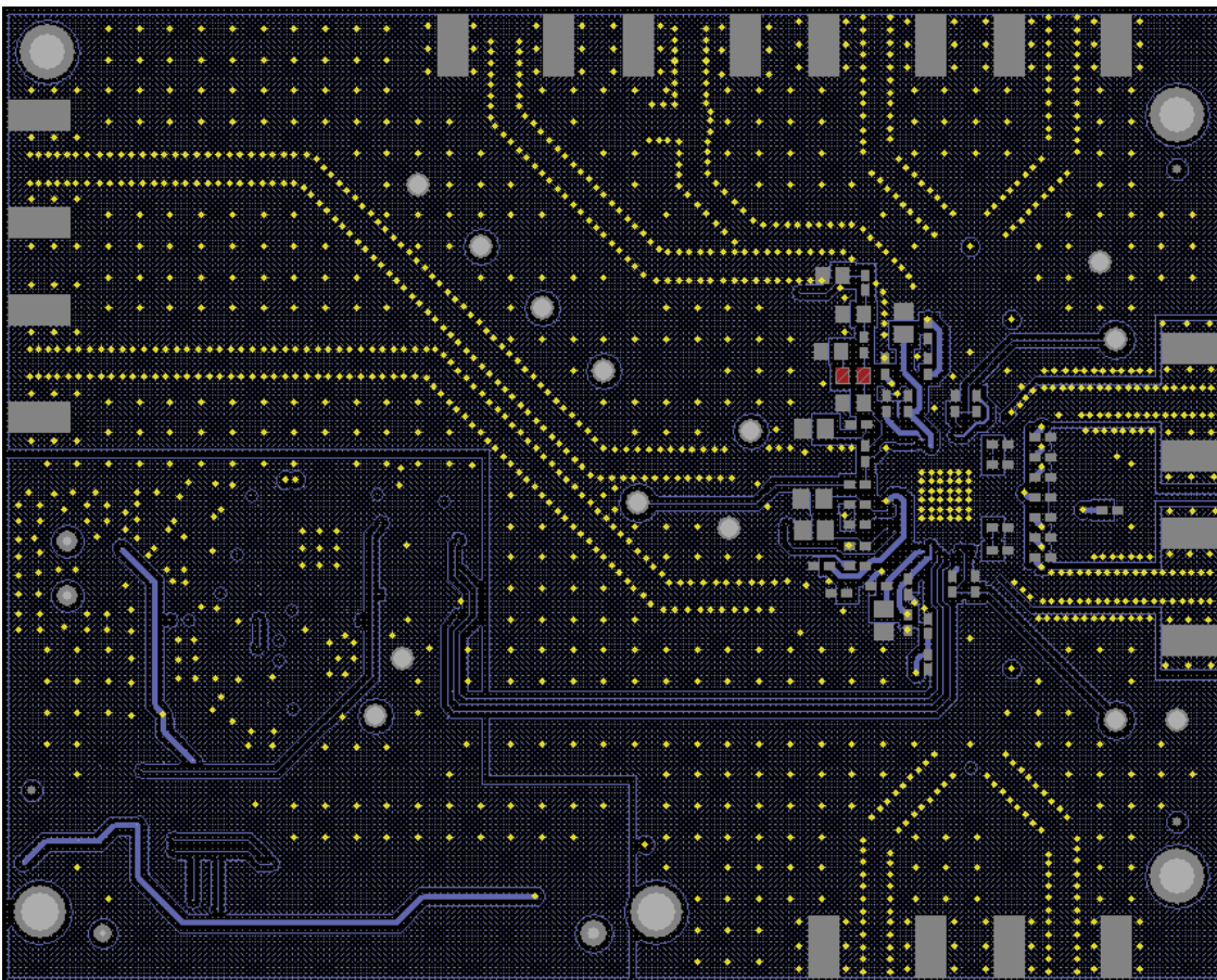
Figure 106. Evaluation Board, Bottom Layer
