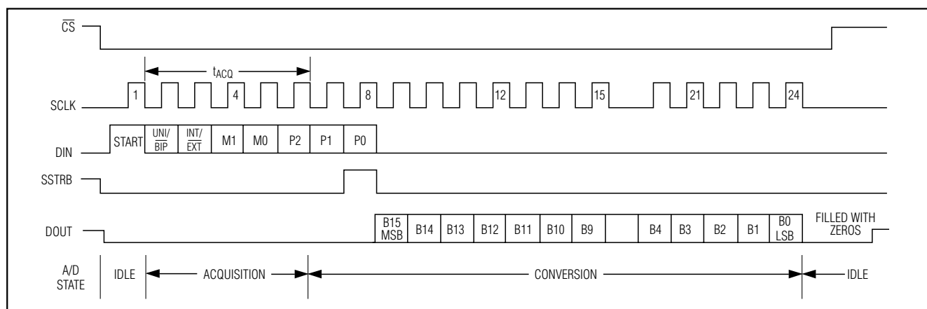
Figure 2. Short Acquisition Mode (24 Clock Cycles) External Clock
