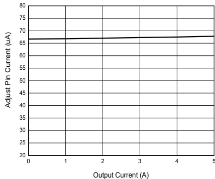
Figure 7. Adjust Pin Current vs. Output Current
