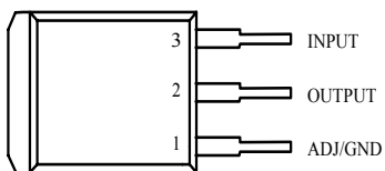
V1 Package (TO-263-3)
