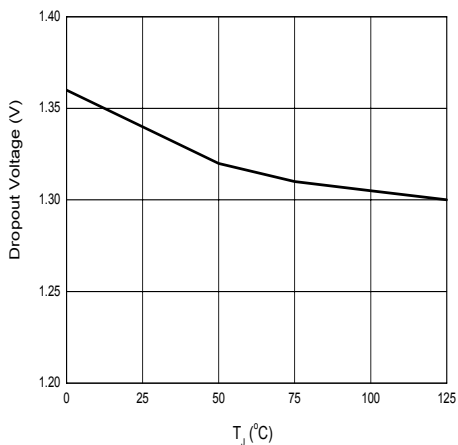
Figure 8. Dropout Voltage vs. Temperature
