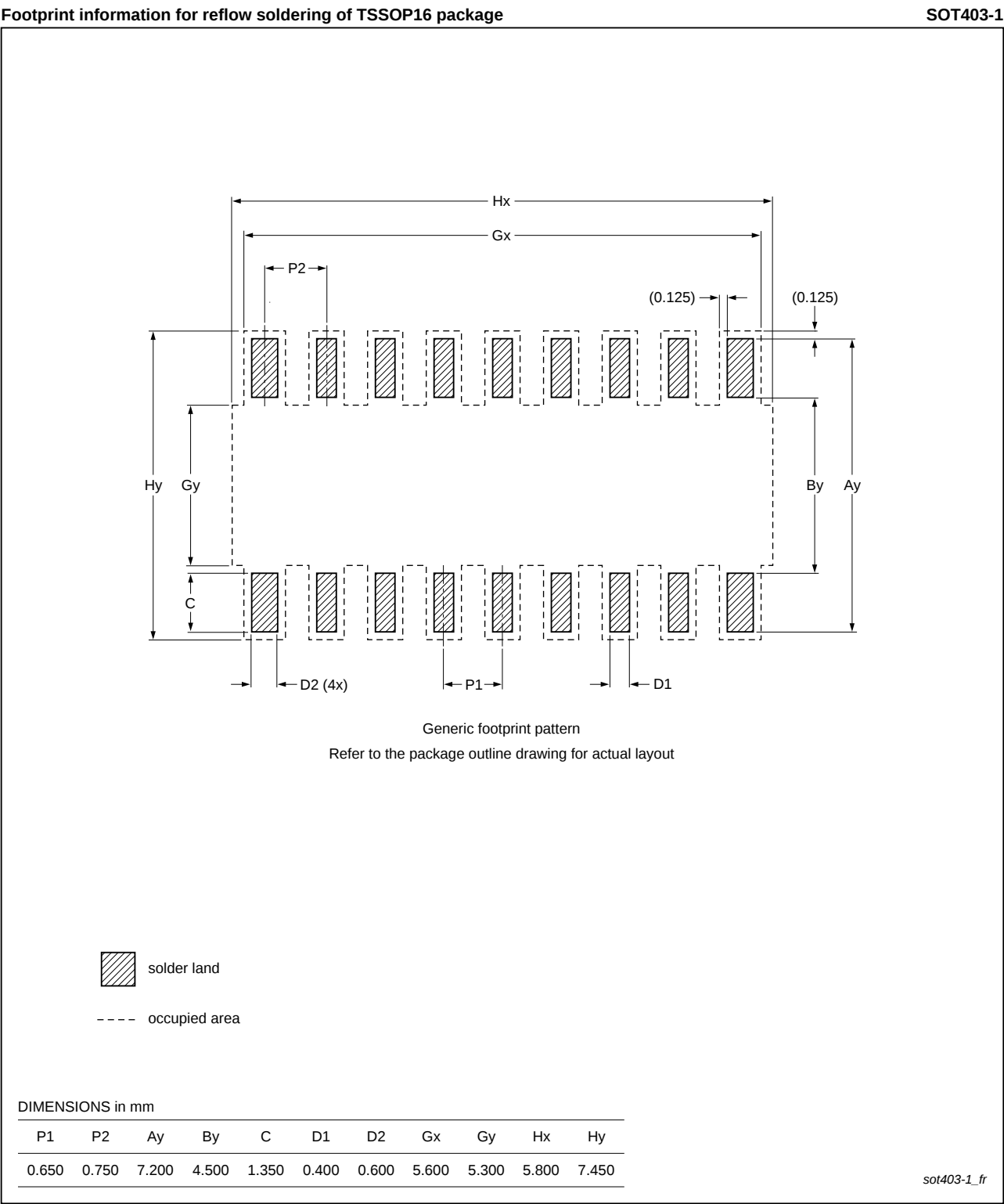
Fig 26. PCB footprint for SOT403-1 (TSSOP16); reflow soldering
