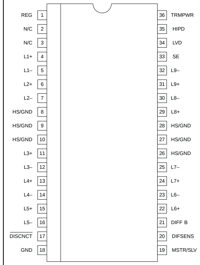
QSOP-36 (Top View) MWP Package
