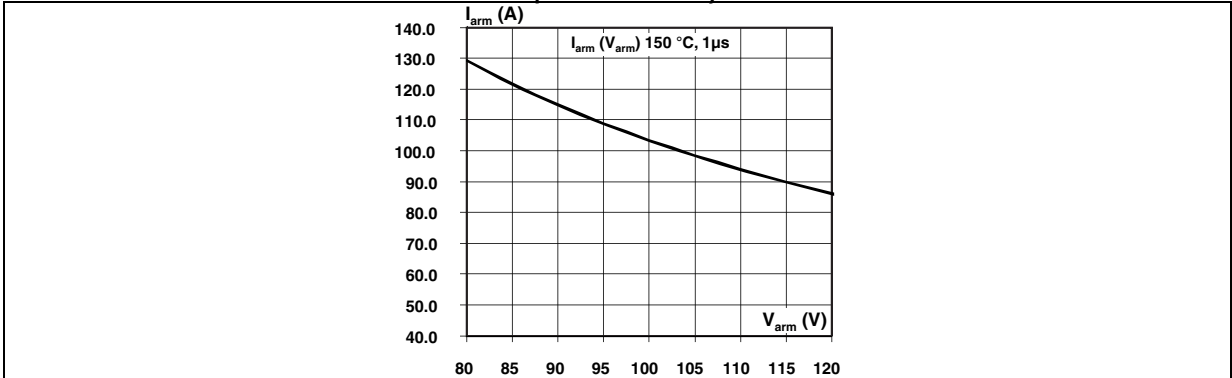
Figure 12. Reverse safe operating area ( t_p < 1\text{ }\mu\text{s} and T_J < 150\text{ }^{\circ}\text{C} )
