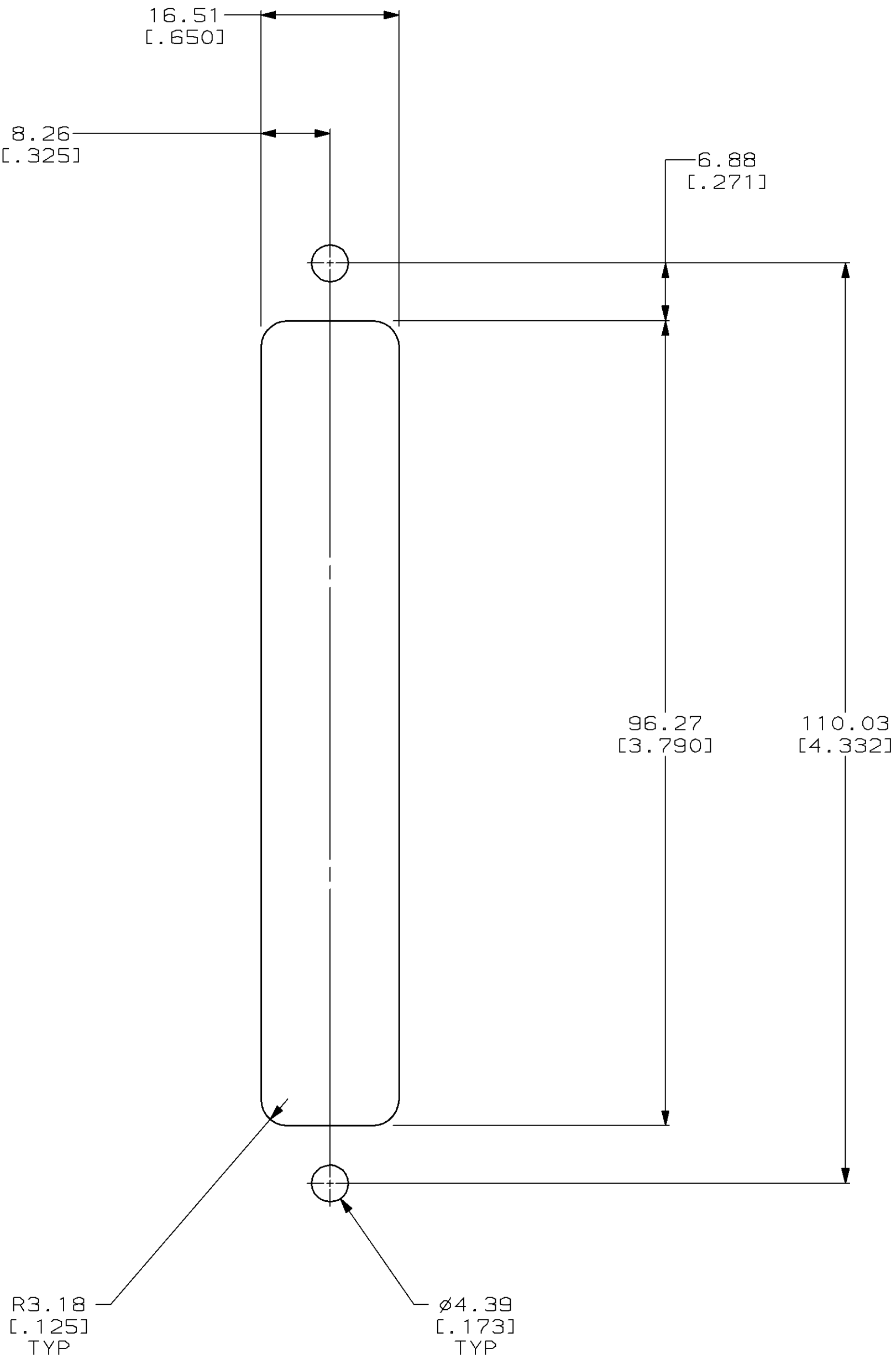
RECOMMENDED PANEL CUTOUT
