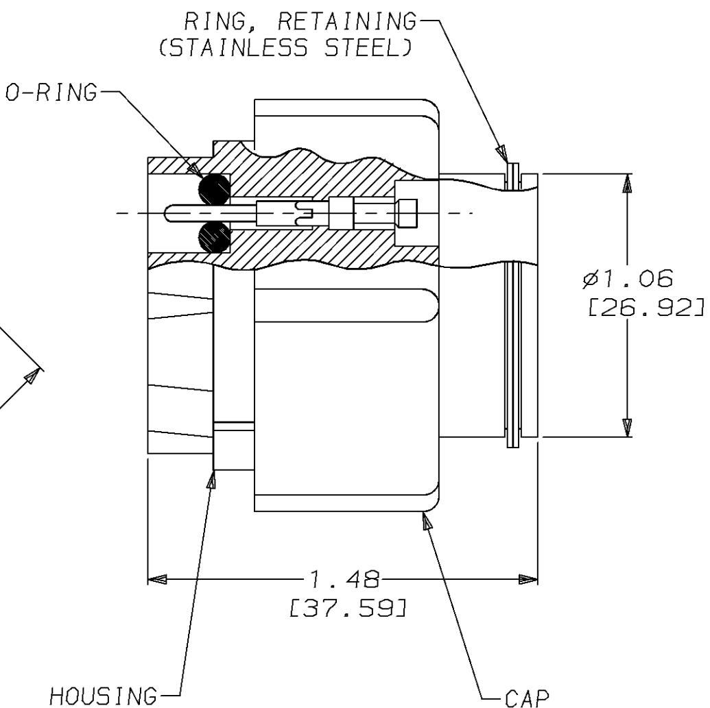
PLUG
