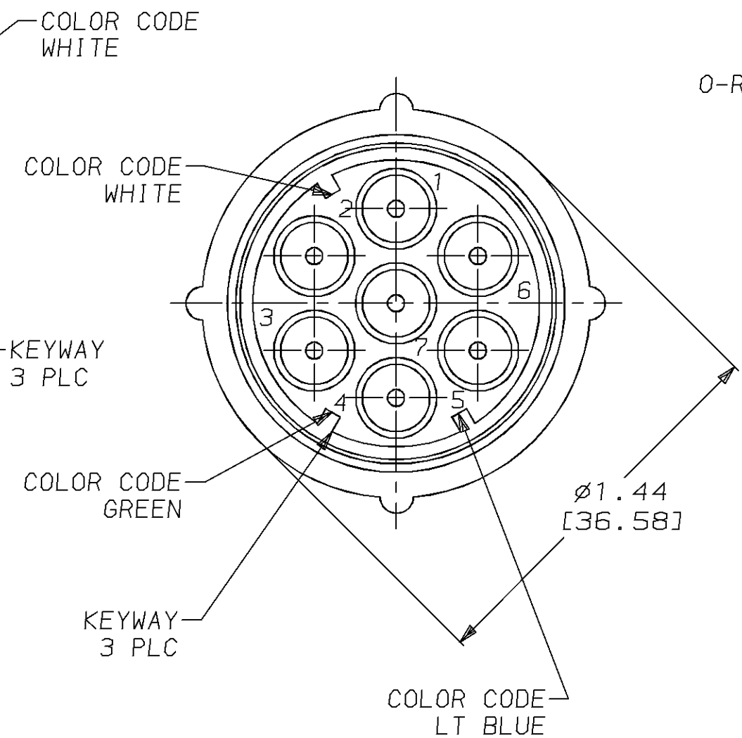
PLUG
