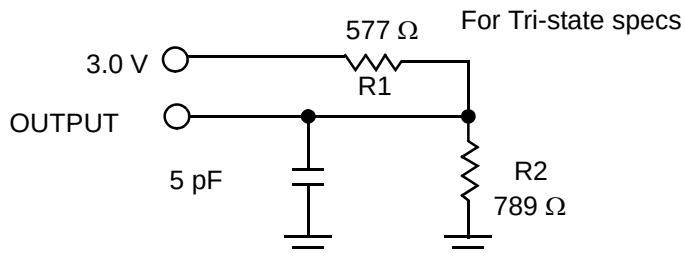
Figure 23. AC Test Loads and Waveforms
