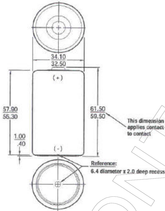
Dimensions (mm)
