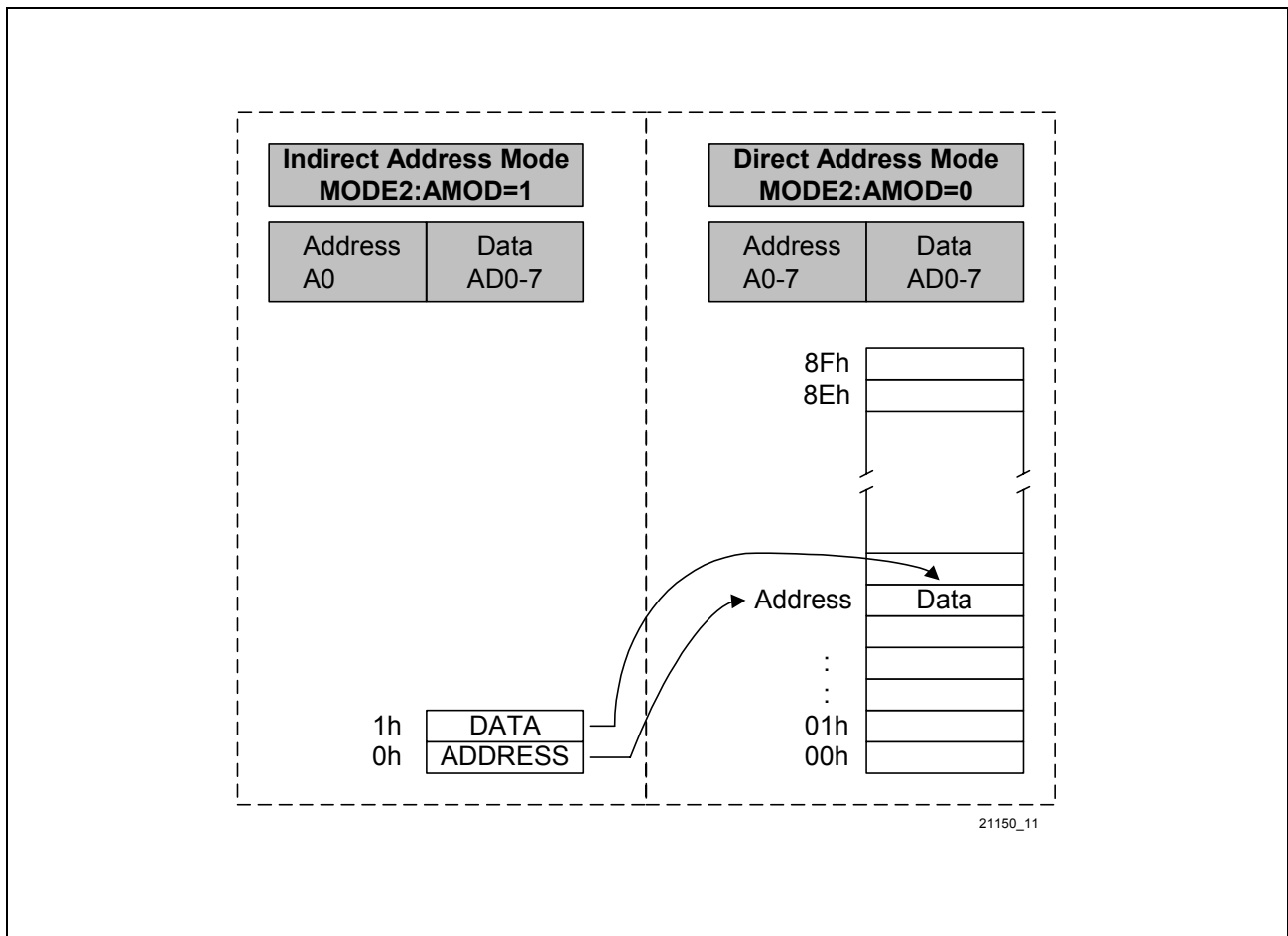
Figure 7 Direct/Indirect Register Address Mode
