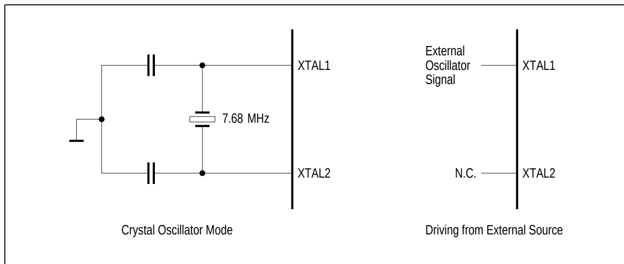
Figure 82 Oscillator Circuits
