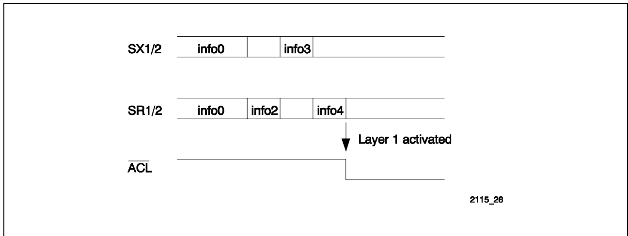
Figure 13 \overline{\text{ACL}} Indication of Activated Layer 1
