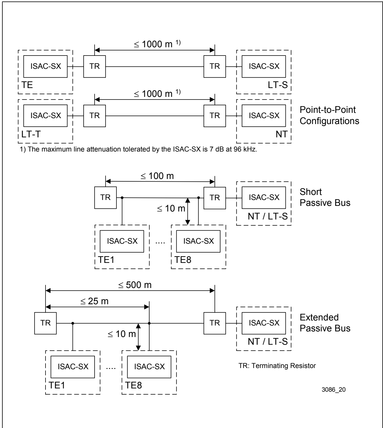
Figure 15 Wiring Configurations in User Premises
