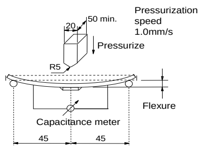
Fig.2 (in mm)
