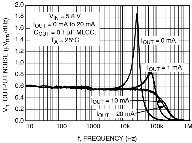
Figure 18. Output Voltage Noise 10 Hz – 1 MHz COUT = 0.1 μF
