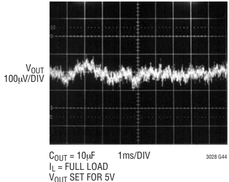
10Hz to 100kHz Output Noise C_{BYP} = 1000pF
