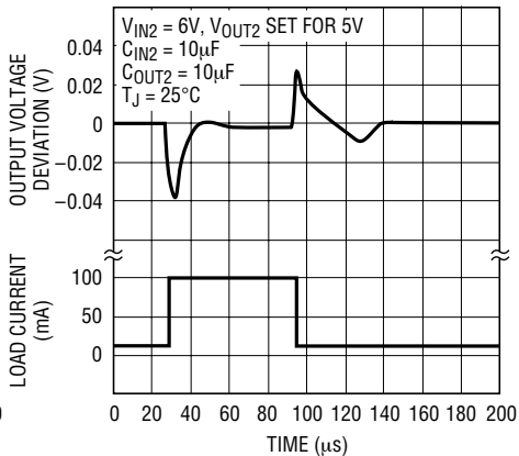
Output 2 Transient Response C_{BYP} = 0.01µF
