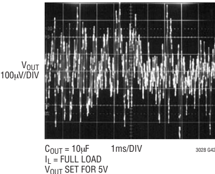
10Hz to 100kHz Output Noise C_{BYP} = 0pF
