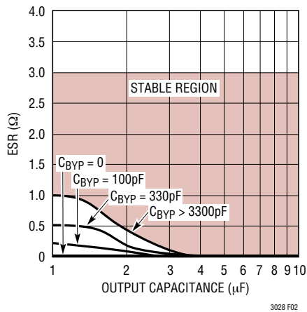
Figure 2. Output 2 Stability
