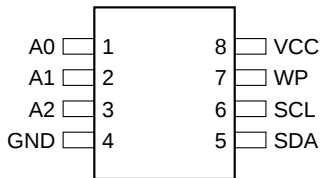
8-Pin SOIC
