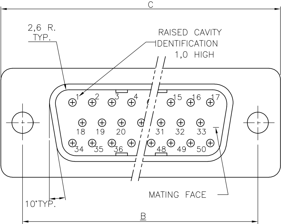
SIZE 5 CONFIGURATION
