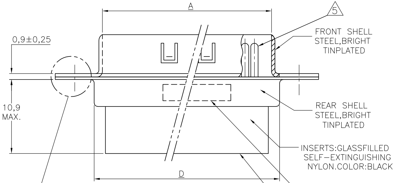
SIZE 5 CONFIGURATION
