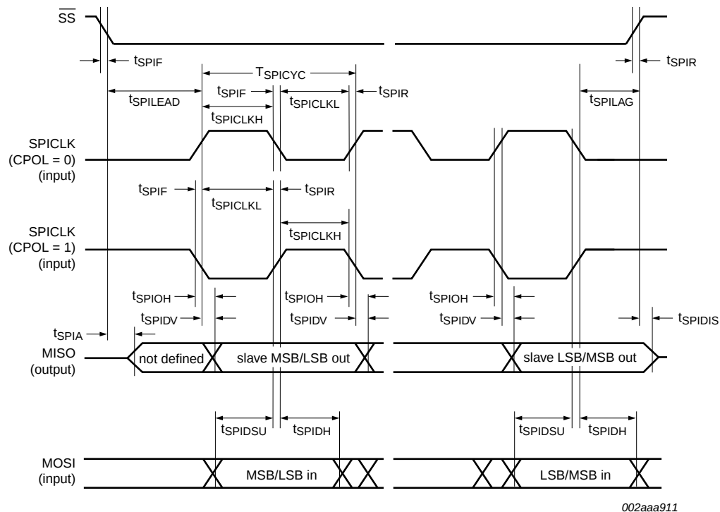
Fig 36. SPI slave timing (CPHA = 1)
