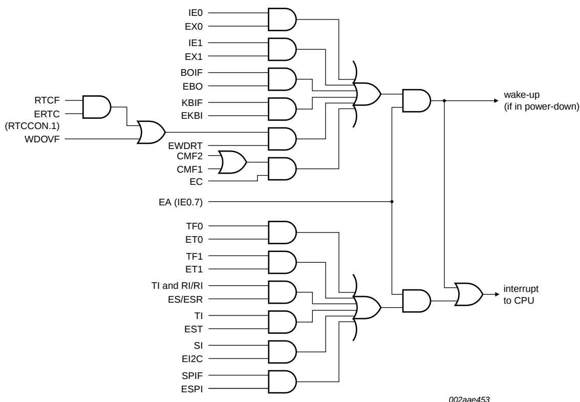
Fig 5. Interrupt sources, interrupt enables, and power-down wake-up sources
