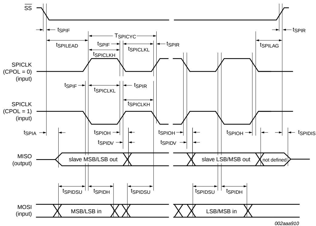
Fig 35. SPI slave timing (CPHA = 0)
