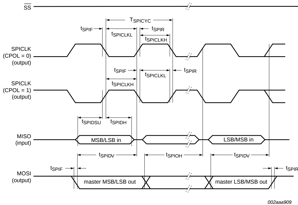
Fig 34. SPI master timing (CPHA = 1)
