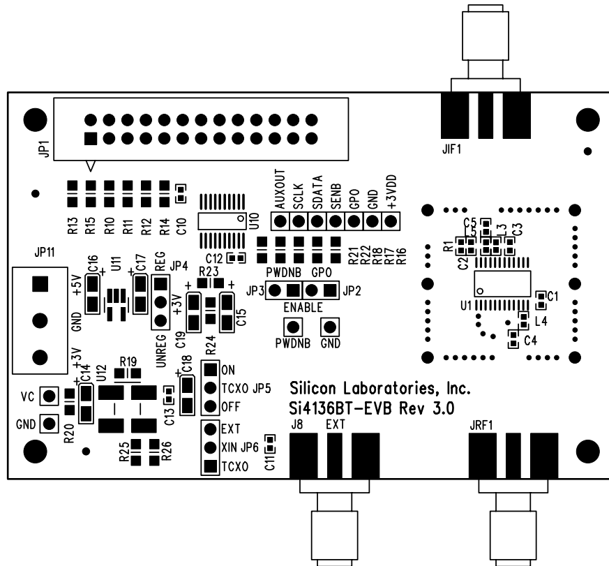
Figure 41. Si4136BT Silkscreen
