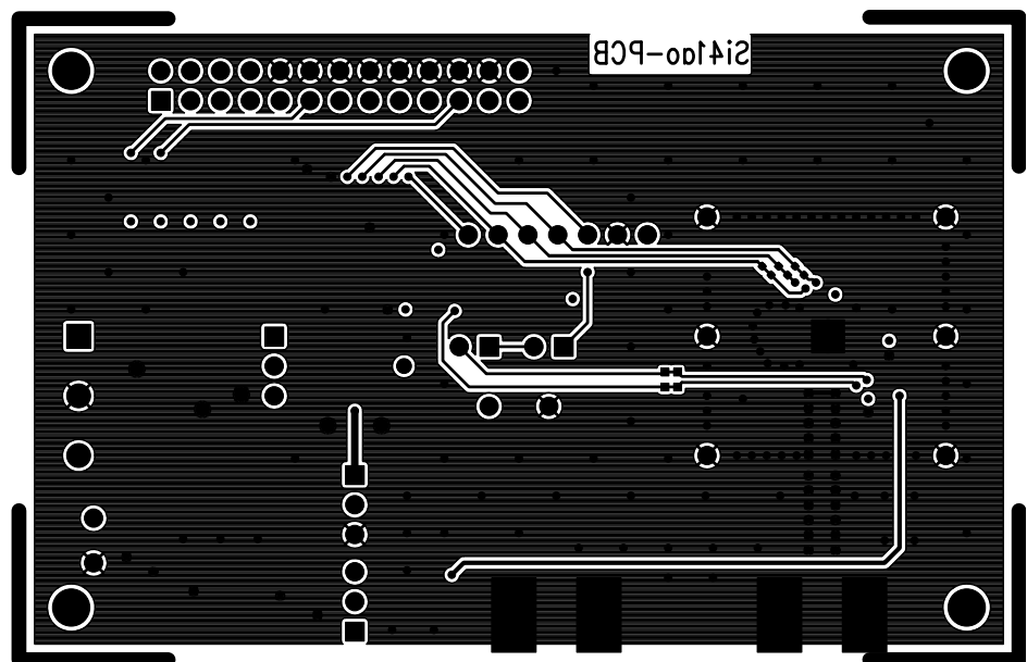
Figure 35. Si4113GX5-BM Solder
