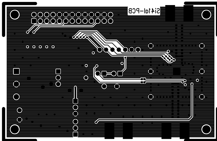
Figure 30. Si4133M Solder
