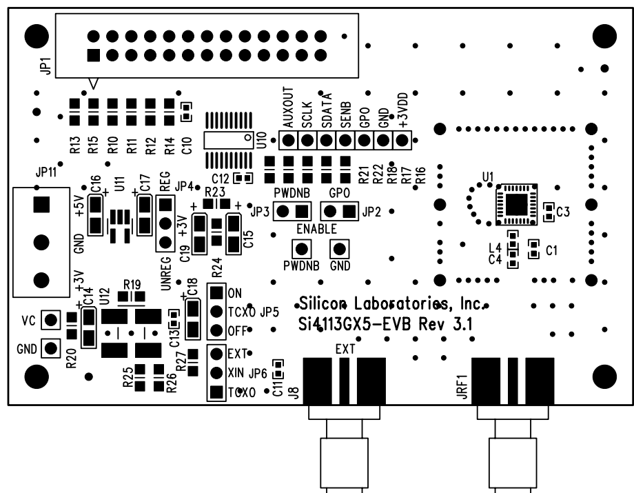
Figure 31. Si4113GX5-BM Silkscreen
