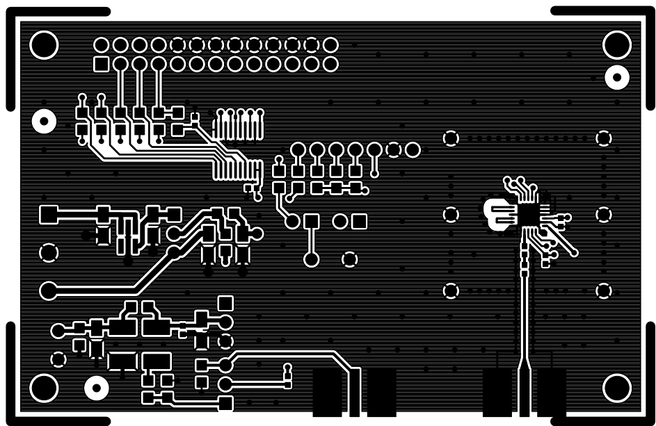
Figure 32. Si4113GX5-BM Component
