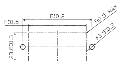
Panel Cutout
