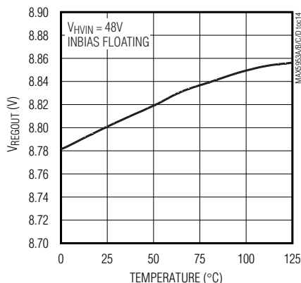
REGOUT VOLTAGE vs. TEMPERATURE
