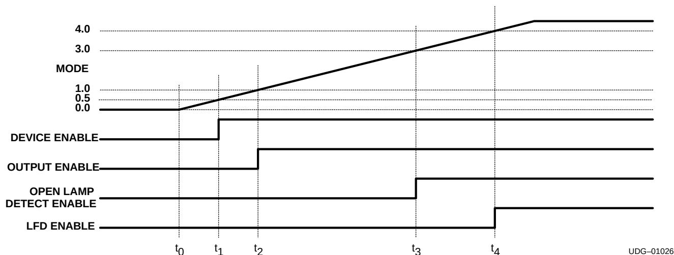
Figure 5. Start-Up Sequence
