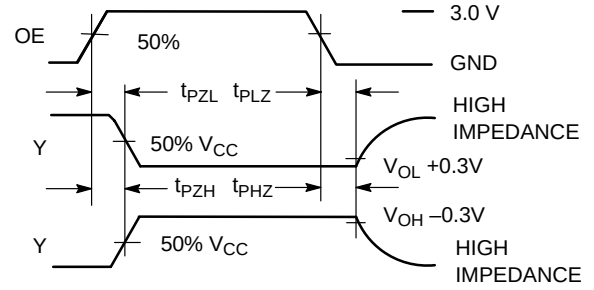
Figure 5. Switching Waveform
