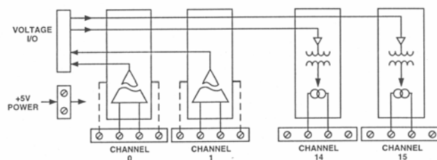
Figure 1 5B01 Functional Block Diagram
