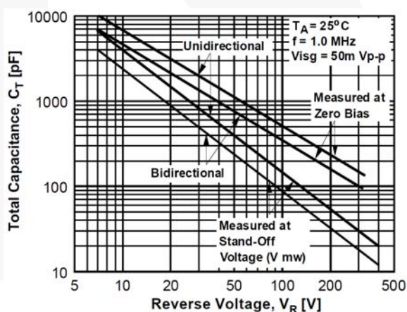
Figure 4. Total Capacitance
