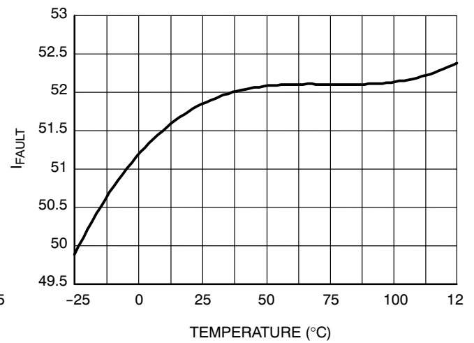
Figure 42. I_{\text{FAULT}} Current Variation versus Junction Temperature (Versions C and D)
