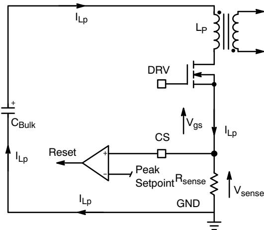
Figure 6. Positive Current-Sense Technique
