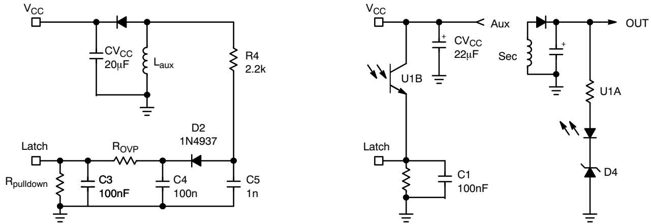
Figure 24. The Latch Input Offers Everything Needed to Implement an OTP Circuit. Another Zener Can Help combining an OVP Circuit if Necessary
