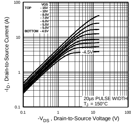
Fig 13. Typical Output Characteristics, T_J = 150^\circ\text{C}
