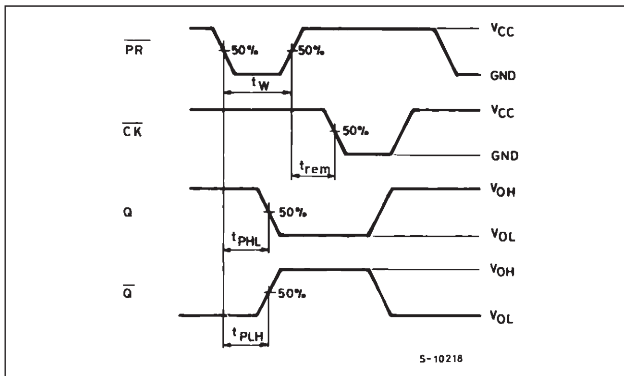
WAVEFORM 2 : MINIMUM PULSE WIDTH ( \overline{\text{PR}} ), REMOVAL TIME ( \overline{\text{PR}} to \overline{\text{CK}} ) (f=1MHz; 50% duty cycle)
