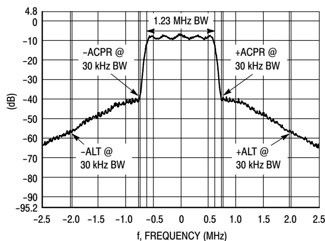
Figure 10. Typical CDMA Spectrum
