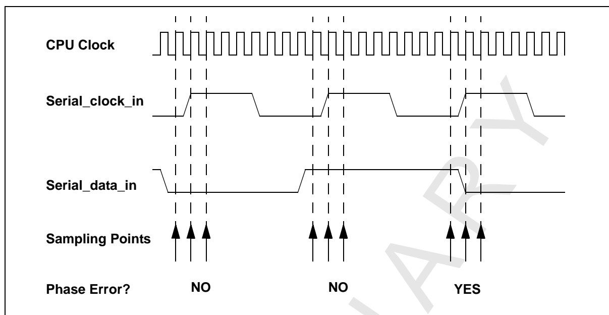
Figure 68: Phase Error Detection
