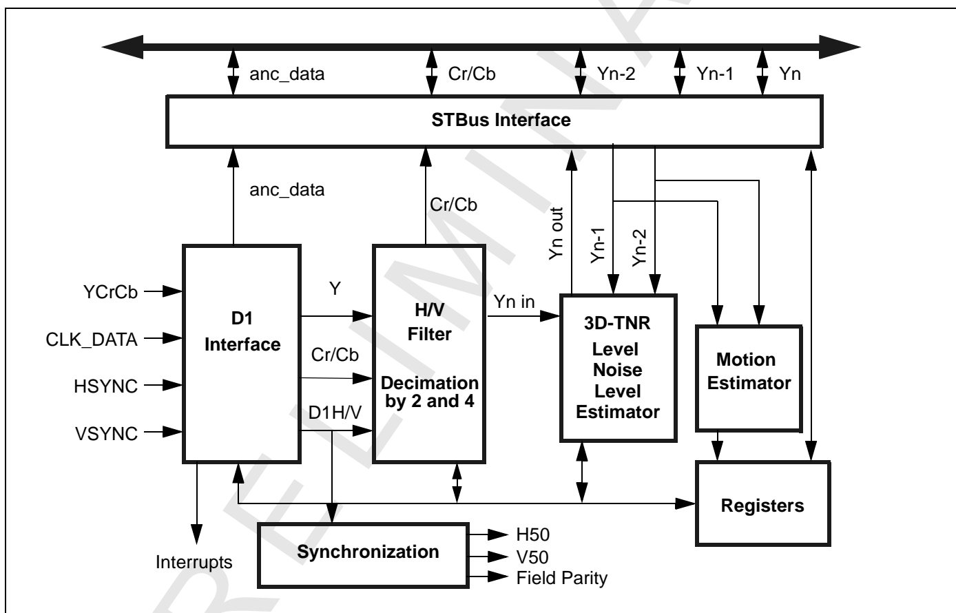
Figure 7: SDIN Block Diagram
