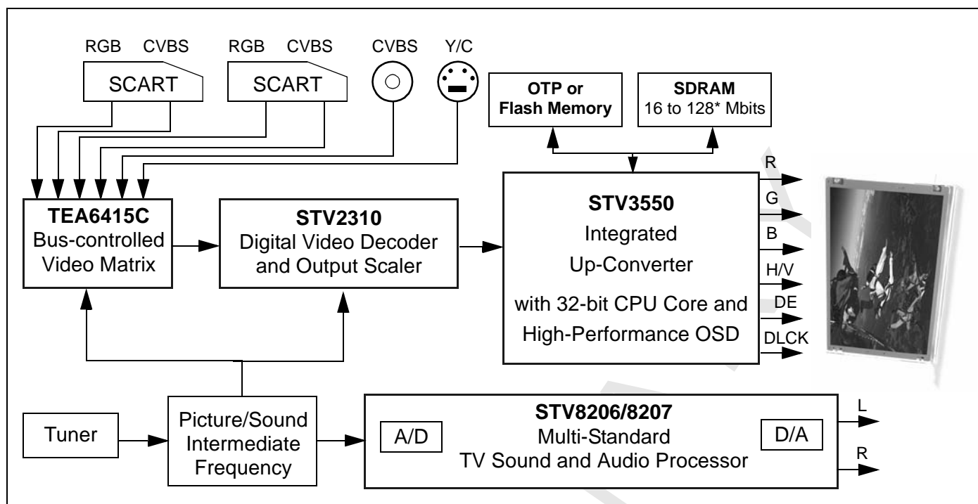
Figure 2: CTV100-LCD Platform Diagram Example
