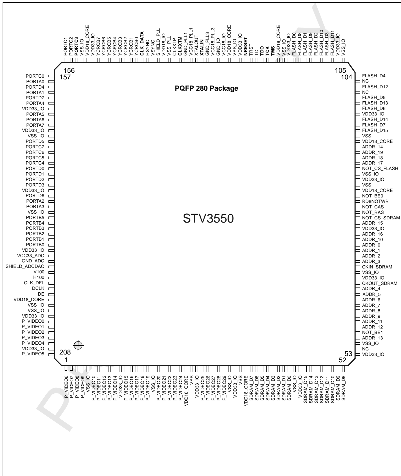
Figure 5: Pinout Diagram
