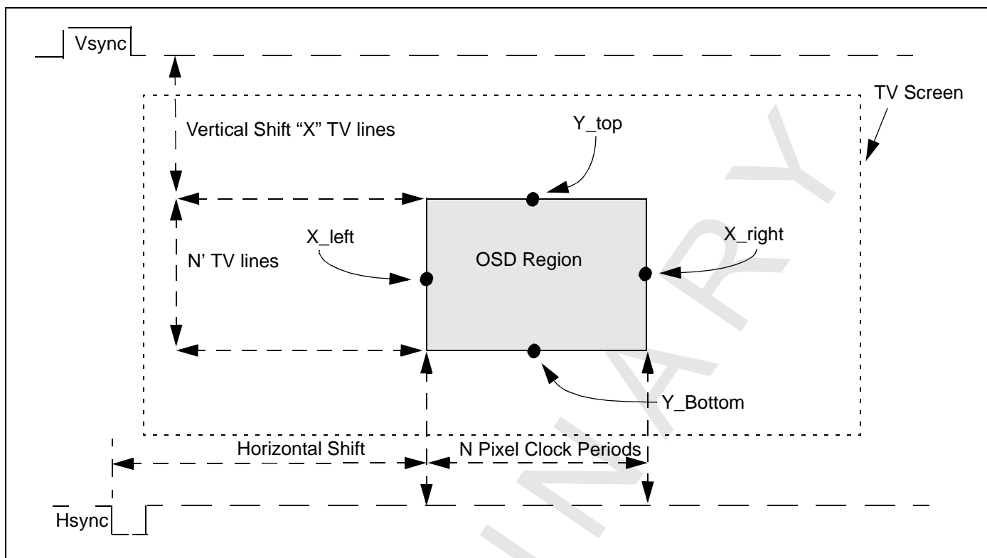
Figure 32: OSD Region Positions
