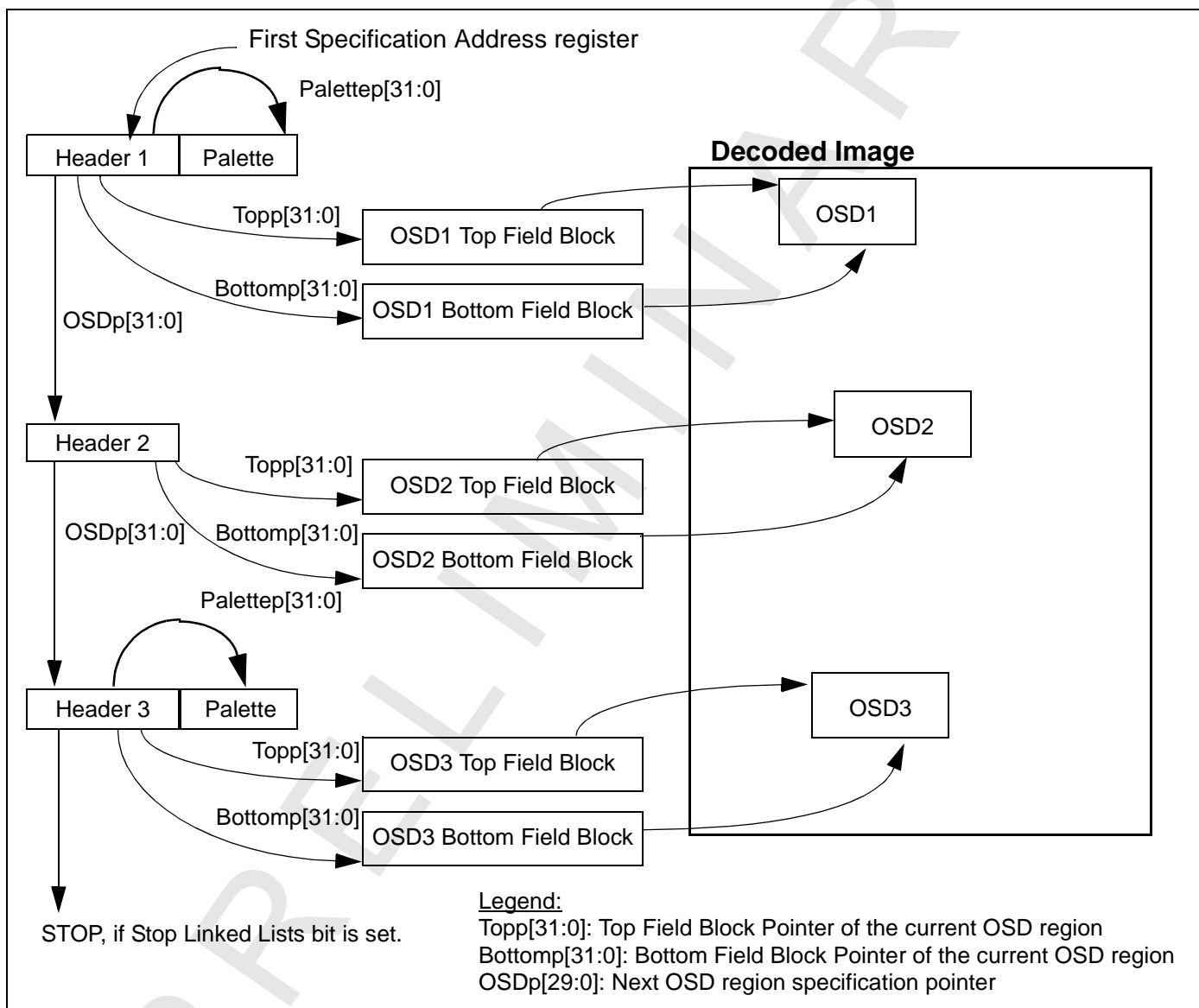
Figure 29: Linked List Structure for OSD Data
