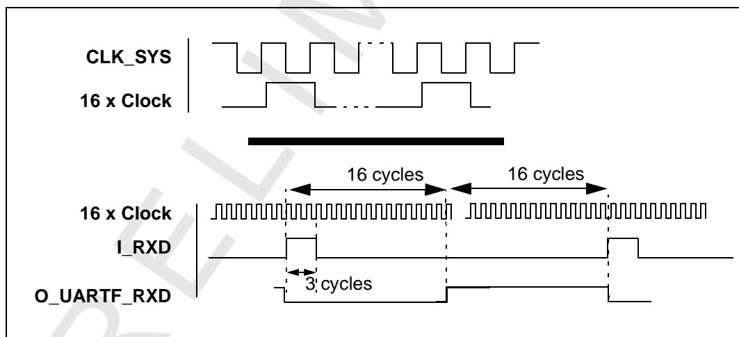
Figure 78: IrDA Decoding Scheme
