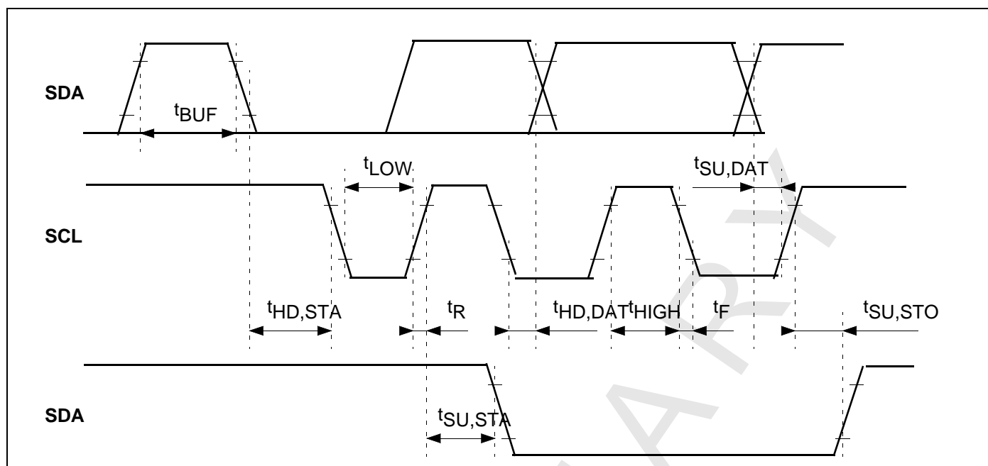
Figure 81: I 2 C Bus Timing
