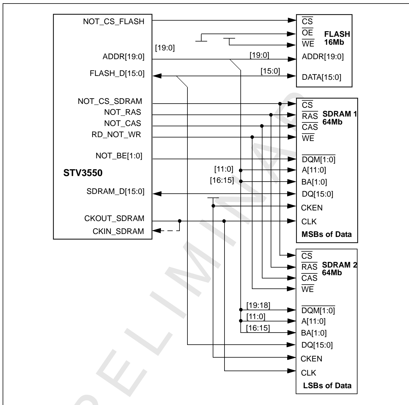
Figure 51: Mixed Configuration using 2 SDRAM Devices
