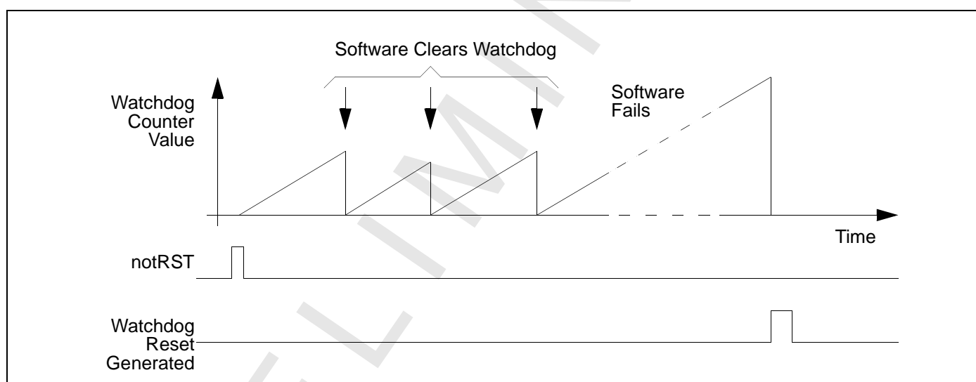
Figure 57: Watchdog Timer Behavior
