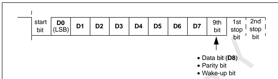
Figure 72: 9-bit Tx Data Frame Format
