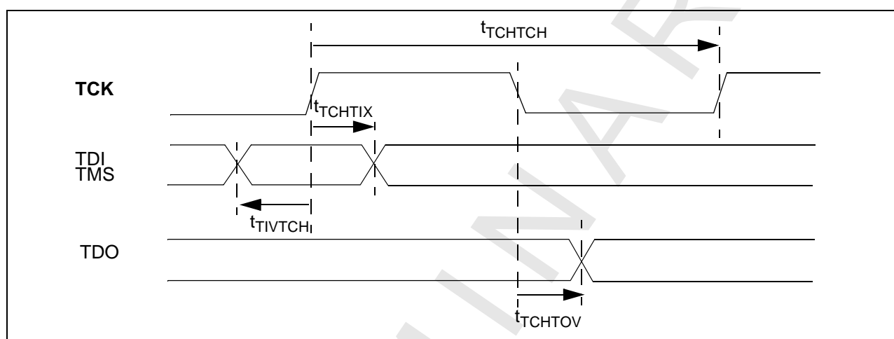
Figure 85: TAP Timings
