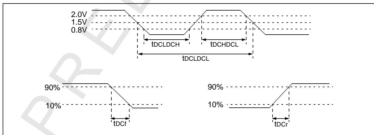
Figure 84: XTALIN Timings
