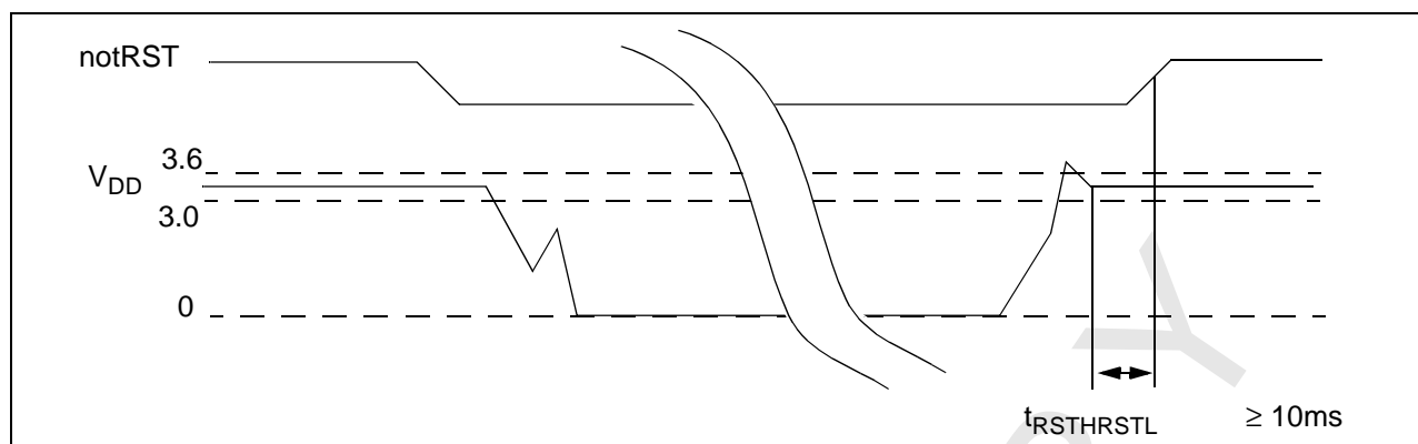
Figure 83: Reset Timings
