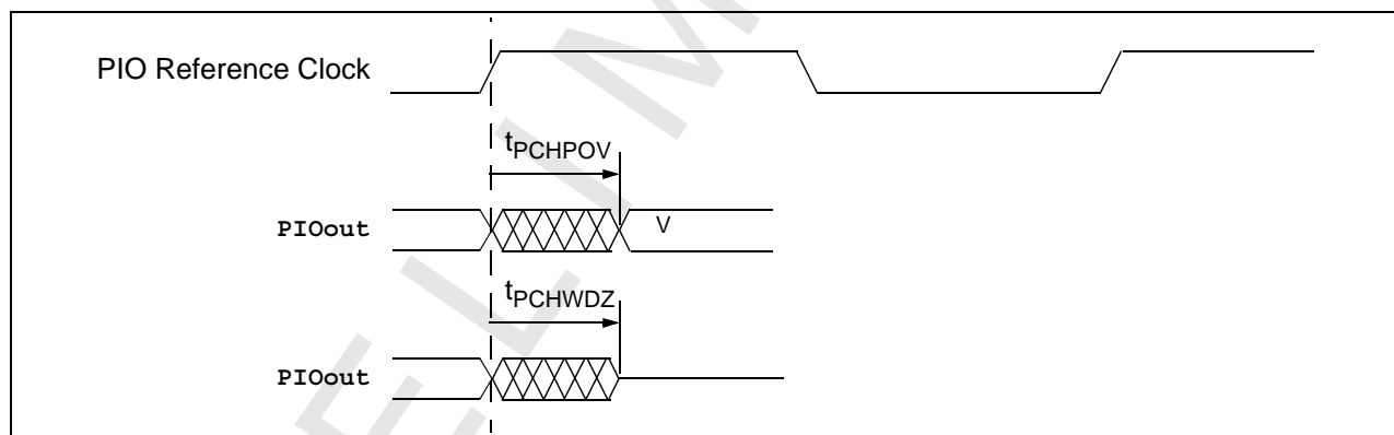
Figure 82: PIO Timings
