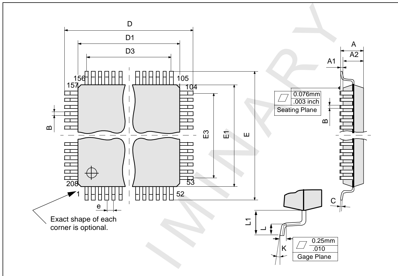
Figure 79: 208-pin Plastic Quad Flat Package
