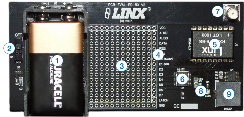
Figure 4: ES Receiver Evaluation Board
