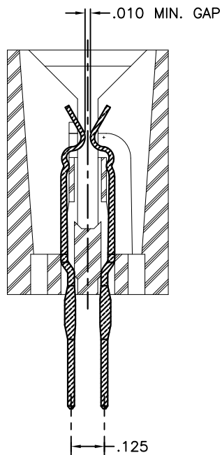
INNER CONTACTS
