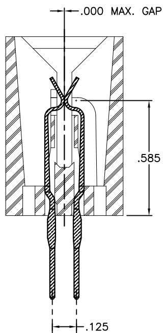
SHORTING CONTACTS
