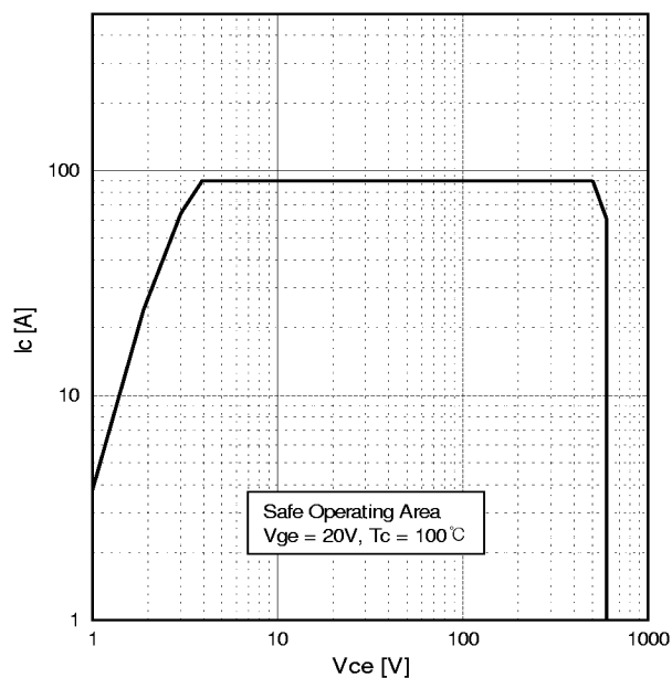
Fig.11 Turn-off SOA
