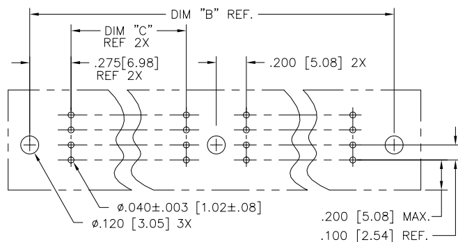
RECOMMENDED PCB LAYOUT (ALL HOLES LOCATED ON .100/2.54 GRID UNLESS OTHERWISE SPECIFIED)
