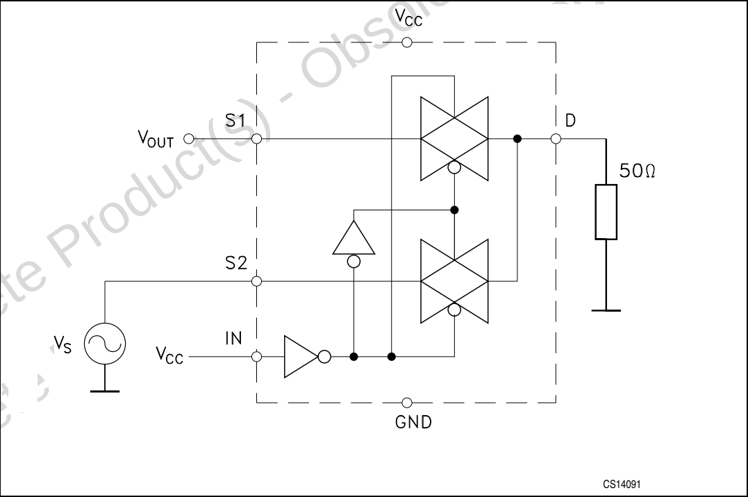
Figure 7. Switch-to-switch crosstalk
