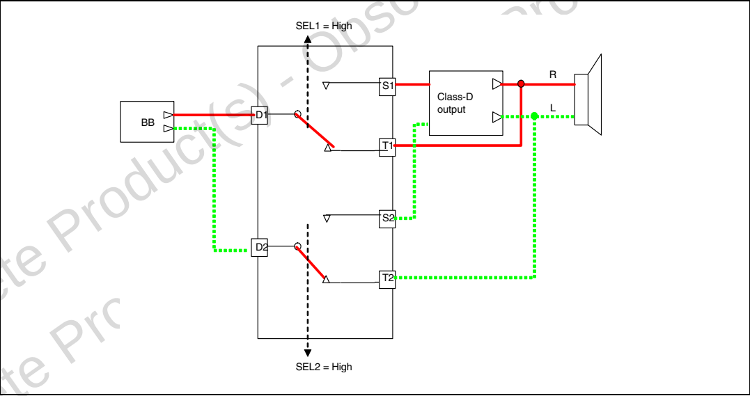
Figure 13. Application diagram
