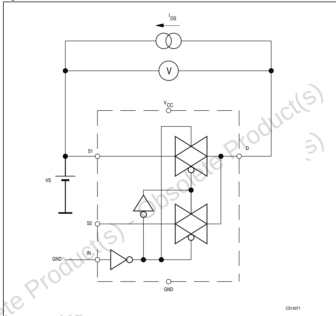
Figure 3. ON resistance
