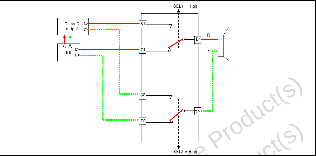
Figure 12. Application diagram
