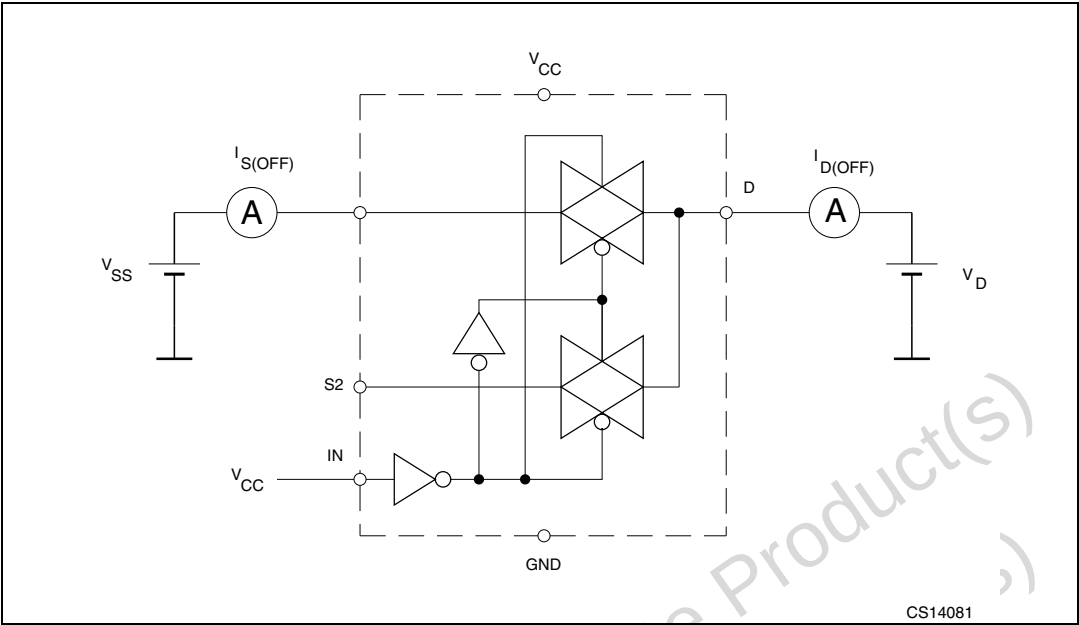
Figure 4. OFF leakage
