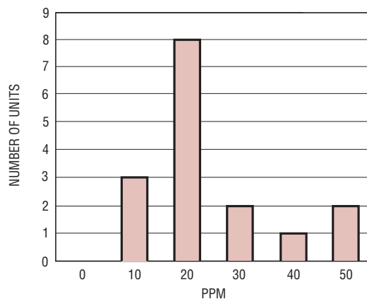
Figure 11. 1X IR Reflow Peak Temperature = 250°C, Delta Output Voltage (ppm)
