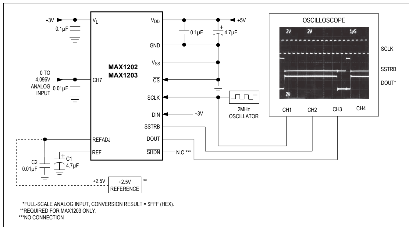
Figure 5. Quick-Look Circuit
