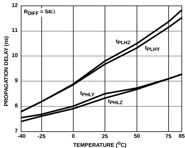
FIGURE 11. DRIVER PROPAGATION DELAY vs TEMPERATURE
