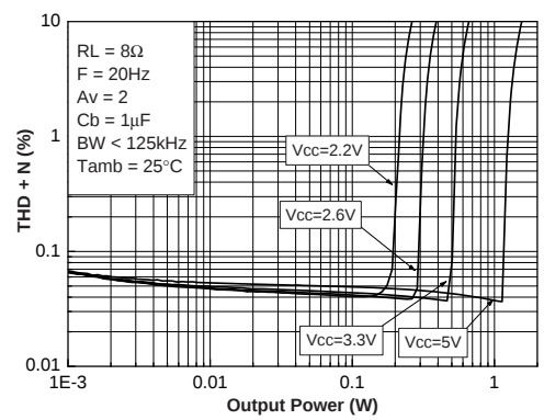
Figure 43. THD + N vs. output power R_L = 8\ \Omega
