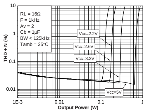
Figure 48. THD + N vs. output power C_b = 1 \mu\text{F}
