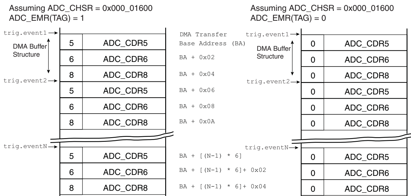
Figure 41-12. Buffer Structure when TSMODE = 0
