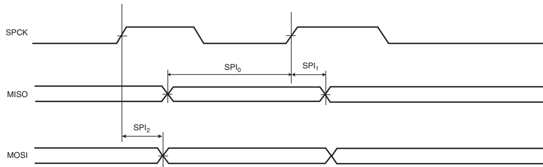
Figure 46-9. SPI Master mode 1 and 2
