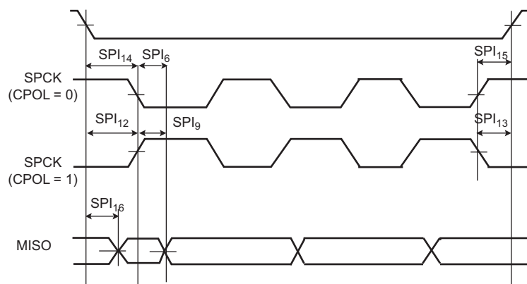
Figure 46-13. SPI Slave mode - NPCS timings
