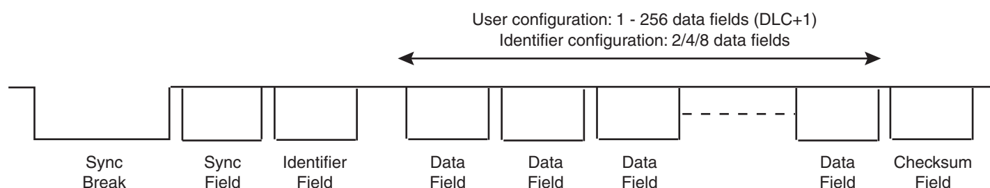
Figure 39-43. Response Data Length
