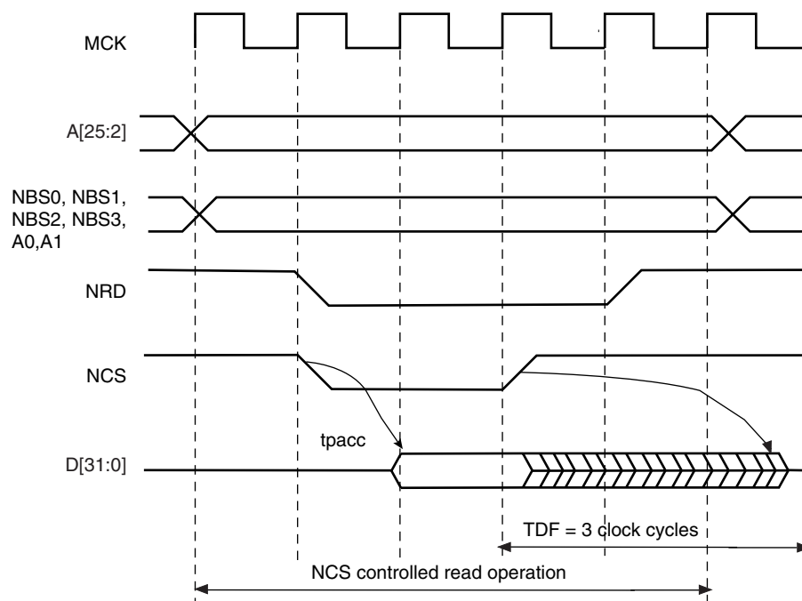
Figure 29-21.TDF Period in NCS Controlled Read Operation (TDF = 3)
