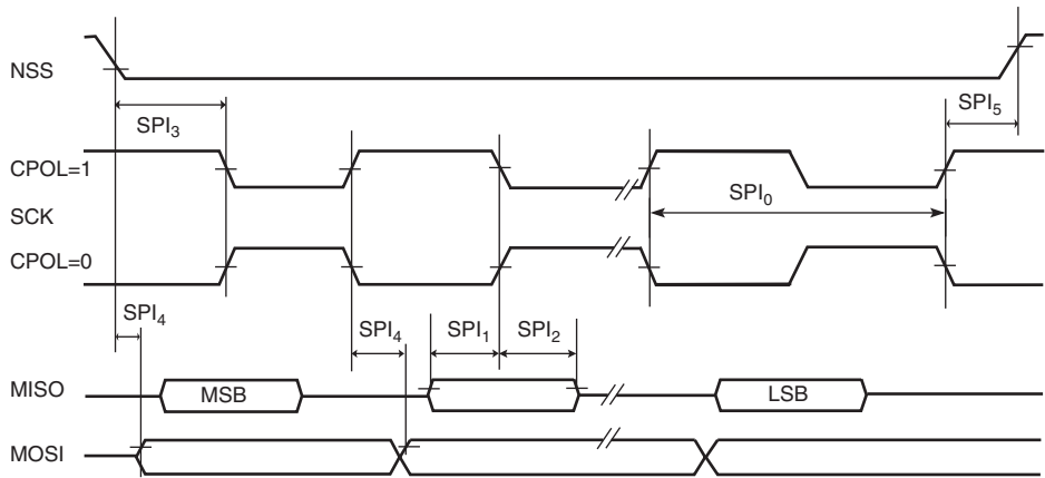
Figure 46-26.USART SPI Master Mode
