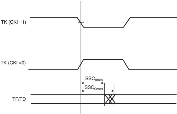
Figure 46-23.Minimum and Maximum Access Time of Output Signals
