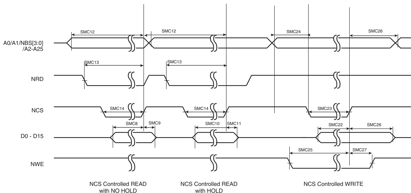
Figure 46-7. SMC Timings - NCS Controlled Read and Write
