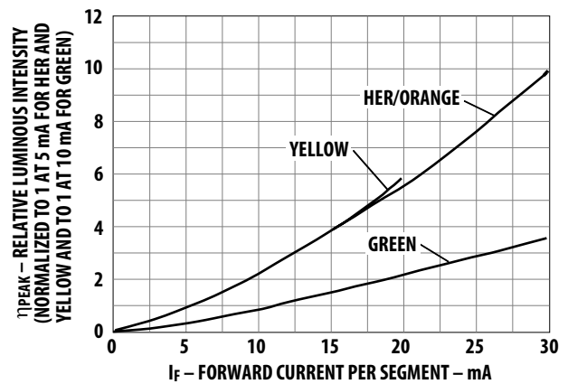
Figure 10. Relative Luminous Intensity vs. DC Forward Current.
