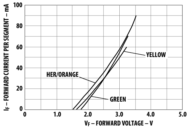
Figure 9. Forward Current vs. Forward Voltage Characteristics.
