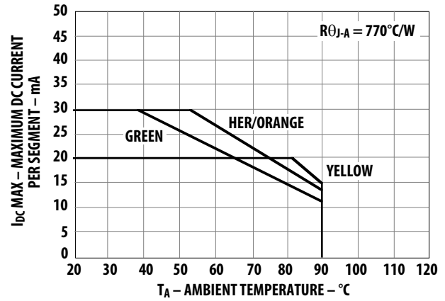
Figure 8. Maximum Allowable DC Current vs. Ambient Temperature.
