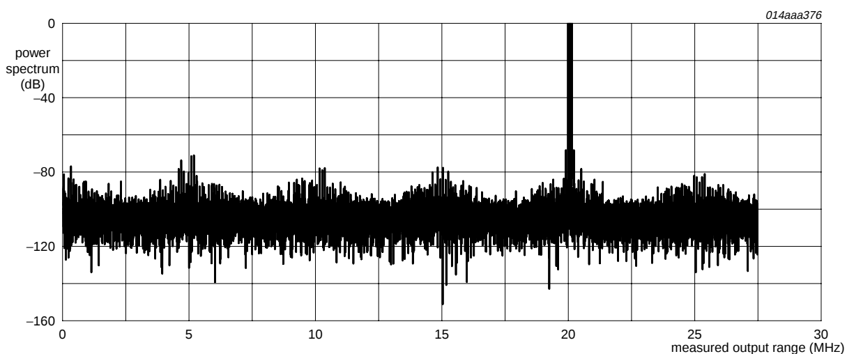
Fig 10. Two-tone; f_{i1} = 20 MHz; f_{i2} = 20.1 MHz; f_{clk} = 55 MHz.
