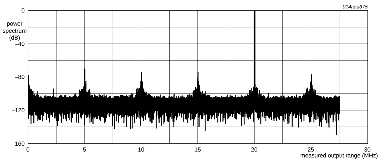
Fig 9. Single-tone; f_i = 20 MHz; f_{clk} = 55 MHz.
