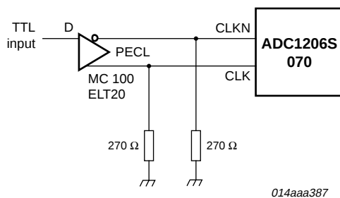
Fig 18. Application diagram for differential clock input PECL compatible using a TTL to PECL translator
