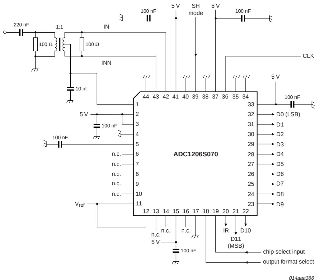
Fig 17. Application diagram
