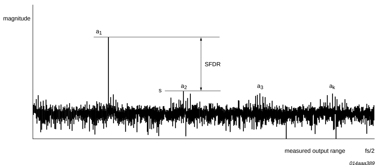
Fig 26. Spectrum of full-scale input sine wave with frequency f_t .
