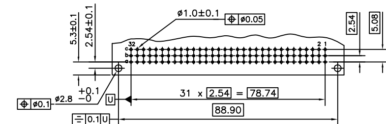
PCB DRILLING DETAILS
