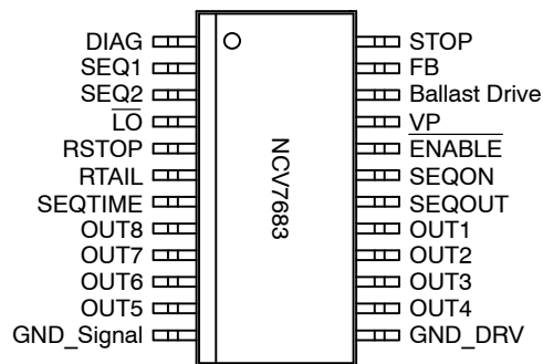
Figure 2. Pinout Diagram
